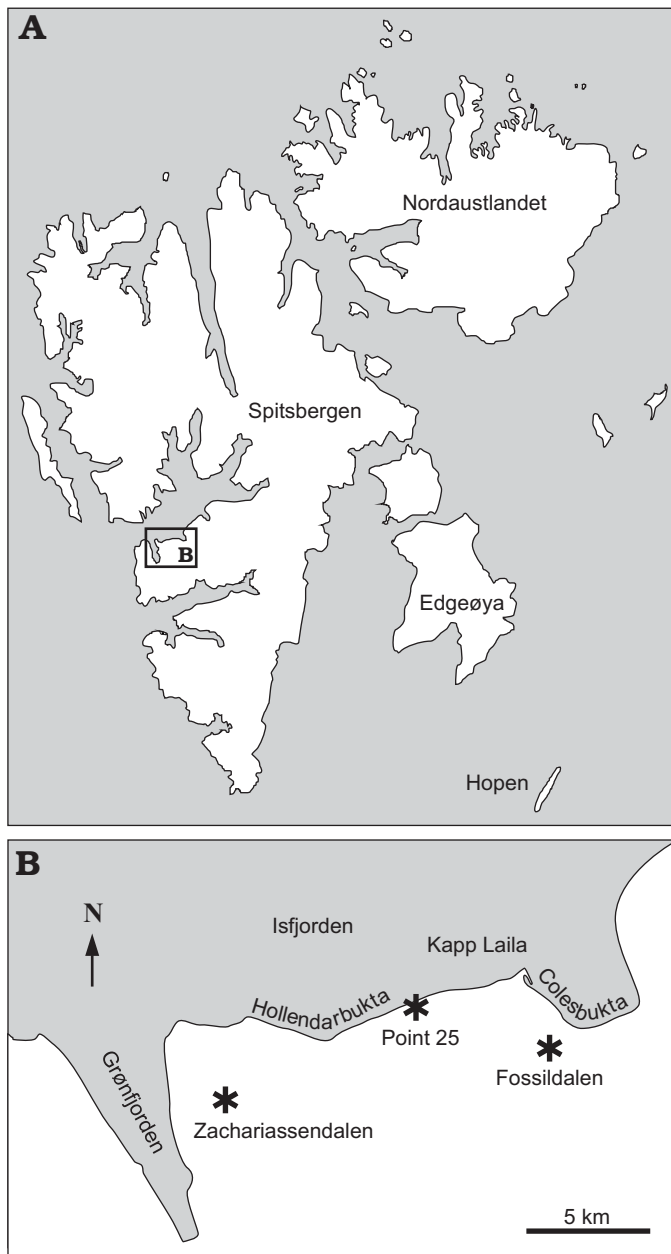
Fig. 1. A. Map of Svalbard showing location of the study area. B. Map of the study area with the fossil localities indicated (asterisks).
