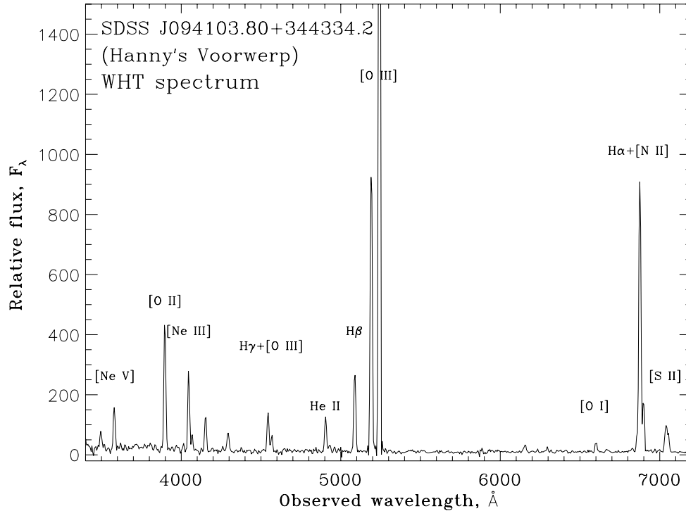
Figure 6. Spectrum of Hanny’s Voorwerp obtained with the WHT, summed over the slit section 15–36 arcsec south of the nucleus of IC 2497. The prominent [O III]4959, 5007 lines dominate the detected emission, while the presence of [Ne V] and [He II] lines indicates that the gas is more highly ionized than can be accounted for by starlight. In order to display the fainter lines, the brightest [O III] line is truncated. Blue and red sections of the spectrum have been merged by resampling to a common wavelength scale, and blended with smoothly varying weights across the range of overlap.
