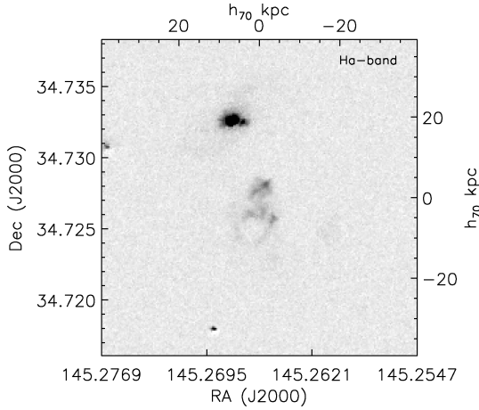
Figure 3. H\alpha emission from the Voorwerp field observed with the KPNO 2.1 m. The Voorwerp itself is prominent. We note also the emission source to the south-west of the IC 2497 nucleus, which is not seen so clearly in any other band.
