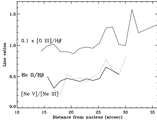
Figure 7. The relationship of three emission-line ratios, each associated with the ionization fraction, with distance from the nucleus of IC 2497. [O III] refers to [O III] \lambda 5007 Å, [Ne V] to [Ne V] \lambda 3426 Å and [Ne III] to [Ne III] \lambda 3869 Å. All change with distance from IC 2497 in the sense indicating increasing ionization level farther from IC 2497, suggesting that the source of the ionization of the Voorwerp has something to do with the neighbouring galaxy (albeit, perhaps, with the details being complicated).
