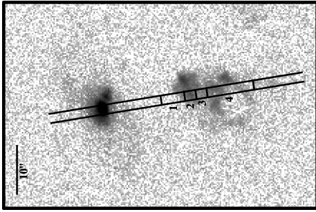
Figure 4. Slit position for both WHT and Lick data plotted on a H\alpha image with non-linear scaling in intensity to show detail in both IC 2497 and the Voorwerp. The regions labelled 1, 2, 3 and 4 correspond to the ‘zones’ in Table 3.
