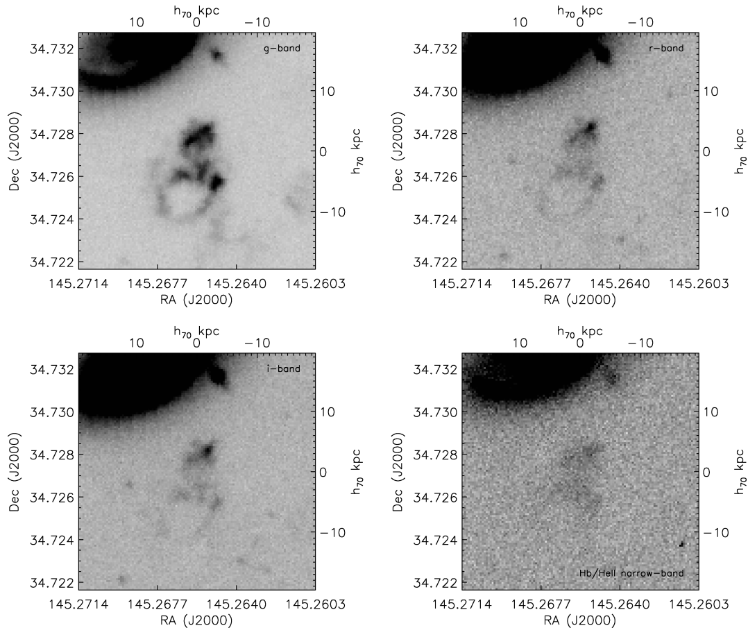
Figure 2. The INT images of the Voorwerp. These g -, r - and i -band images are significantly deeper than the SDSS images in Fig. 1 and were obtained in better seeing conditions. We also present a narrow-band image in the broad \text{H}\beta filter (centred on \lambda = 4861 \text{ \AA} ; FWHM = 170 \text{ \AA} ), which at the redshift of IC 2497 and the Voorwerp traces \text{He II } \lambda 4686 . We also indicate the physical scale in h_{70} kpc at the redshift of the system.
