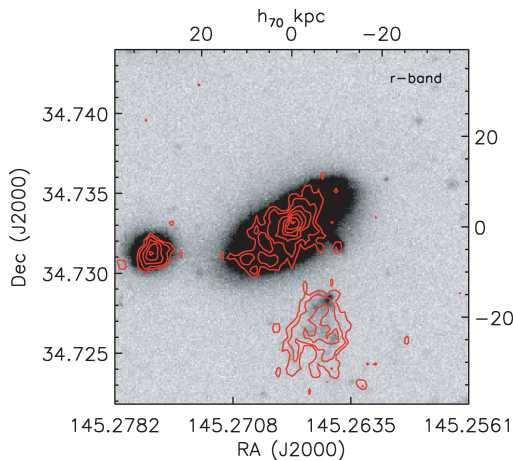
Figure 5. Image of the field obtained after 4700-s exposure with the UV/optical telescope on Swift . The UV data are shown as contours overlaid on a r -band image from SDSS. Both IC 2497 (the central source) and the Voorwerp are strong UV sources.
