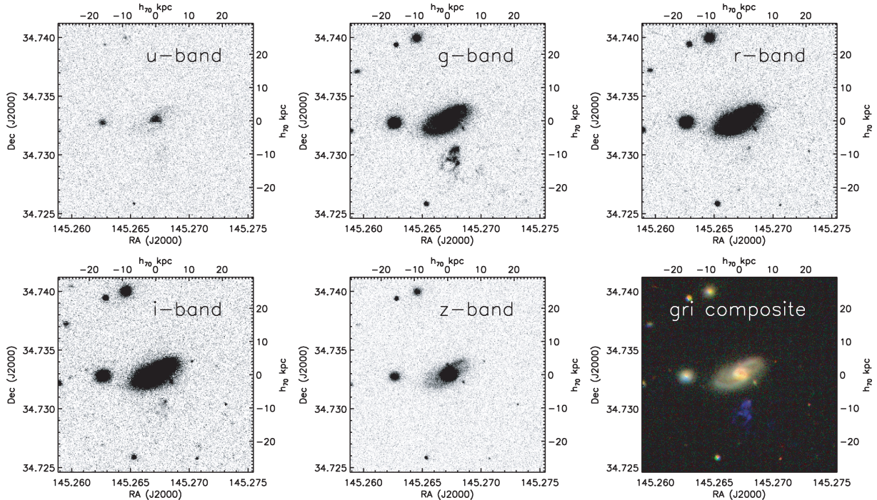
Figure 1. The SDSS images of the main galaxy IC 2497 and the Voorwerp. We show each of the five SDSS images ( u , g , r , i and z ) separately as well as a three-colour gri composite (Lupton et al. 2004). The latter is similar to the Galaxy Zoo image in which the Voorwerp was discovered. IC 2497 is clearly visible in all five bands, while the Voorwerp is strikingly prominent only in the g band. It is marginally detected in the u , r and i bands, and undetected in z . We also indicate the physical scale in h_{70} kpc at the redshift of the system.
