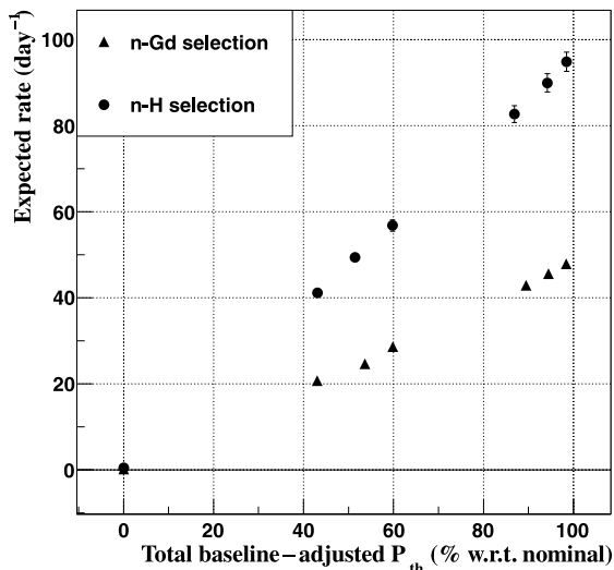
Fig. 1. Expected unoscillated antineutrino event rate as a function of the total baseline-adjusted thermal power ( P_{th}^* = \sum_i^{N_r} P_{th}^i/L_i^2 ), for the n-Gd and n-H analyses. P_{th}^* is presented in percentage of the nominal power.
