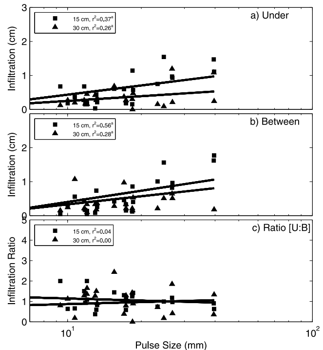
Figure 9. Relation between pulse size and infiltration at depths of 15 and 30 cm (a) under shrubs, (b) between shrubs, and (c) presented as a ratio of under:between shrubs for 32 selected precipitation pulses in 1990–1991 and 2003–2009. Solid lines represent the best fit relation with correlation coefficients given in the legend box. The superscript “a” signifies statistical significance at \alpha < 0.01 .
