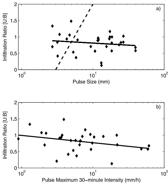
Figure 8. Ratio of infiltration under and between shrubs related to (a) pulse size and (b) maximum 30 min pulse intensity. The solid lines represent the best fit regressions for the Lucky Hills measurements ( r^2 < 0.01 ); the dashed line represents the relation determined by Bhark and Small [2003] for similar measurements at the Sevilleta National Wildlife Refuge.
