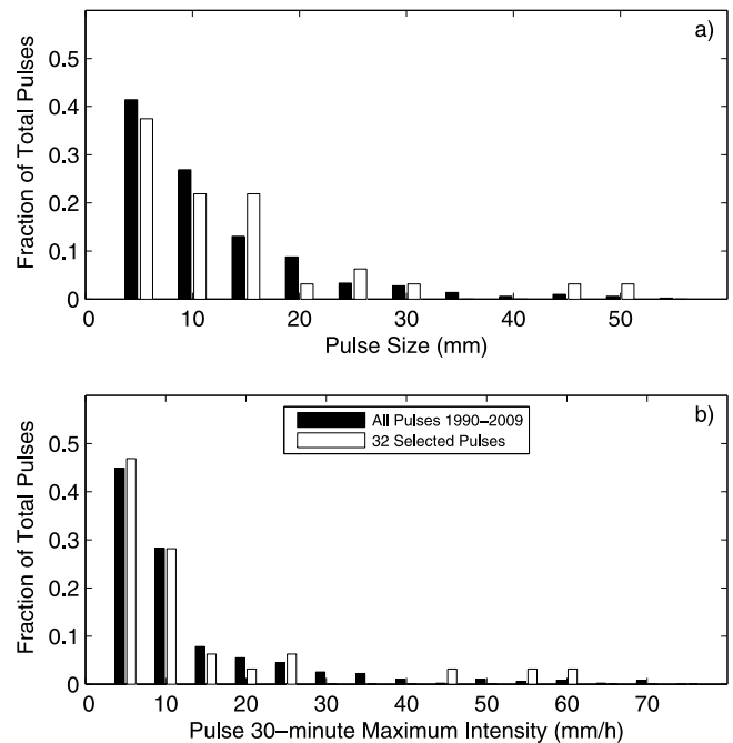
Figure 2. Frequency distributions of (a) pulse size (mm) and (b) 30 min maximum intensity (mm/h) for pulses > 2 mm over the study period 1990–2009 ( n = 513 ) and the 32 selected pulses (Table 3).
