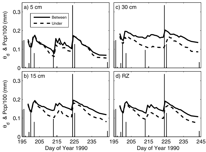
Figure 4. Trends in root-zone soil moisture under and between shrubs after a summer precipitation pulses in 1990 at depths of (a) 5 cm, (b) 15 cm, (c) 30 cm, and (d) through the root zone (to 30 cm).
