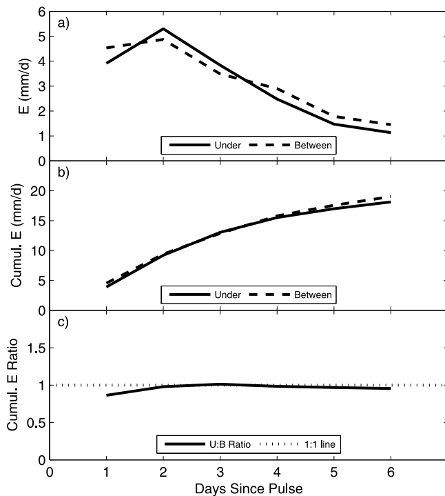
Figure 6. Pulse-related (a) evaporation rates, (b) cumulative evaporation, and (c) under:between ratio of cumulative evaporation measured by microlysimeters located under and between shrubs at Lucky Hills on days since pulse in 2009.
