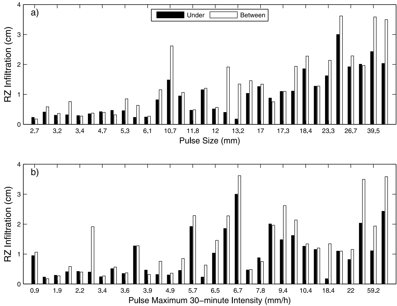
Figure 7. Root-zone infiltration under and between shrubs for 32 selected precipitation pulses in 1990–1991 and 2003–2009, sorted by (a) pulse size and (b) maximum 30 min pulse intensity. The average infiltration values for all pulses are summarized in Table 5.
