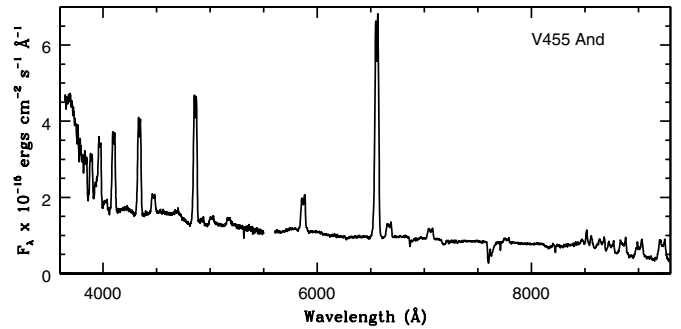
Figure 2. APO spectra obtained 2010 October 2. Short gap near 5500 Å marks where the dichroic separates the blue and red spectra.
