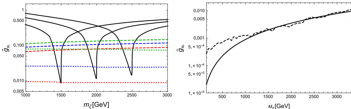
Figure 5. Left panel: same as the left panel in figure 3 but with the future reach by the High-Luminosity LHC with a 3000/fb luminosity and the LUX-ZEPLIN DM experiment. Right panel: same as the right panel in figure 4 but for the future reach.
