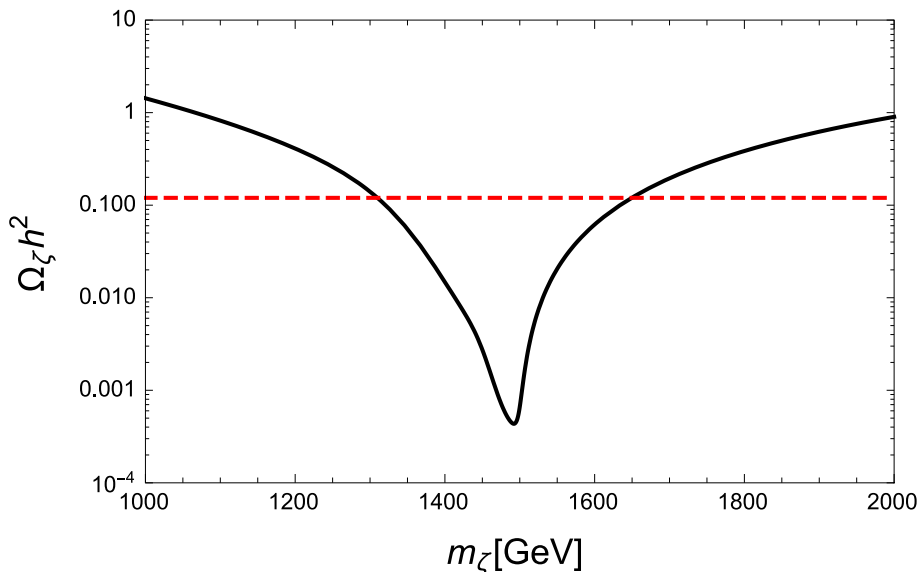
Figure 2. A sample plot of DM relic density vs. m_\zeta for g_\zeta = \tilde{g}_{BL} = 0.2 and M_X = 3 TeV, along with the observed relic density (dashed horizontal line).
