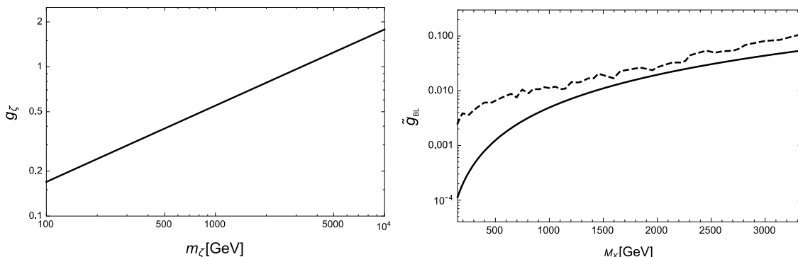
Figure 4. Left panel: plots of g_\zeta vs m_\zeta along which the observed DM relic abundance is reproduced. Here, we have set M_X = m_\zeta/3 . Right panel: upper bounds on \tilde{g}_{BL} as a function of M_X along the solid line in the left panel. The solid and dashed lines correspond to the XENON1T and the ATLAS bounds, respectively.
