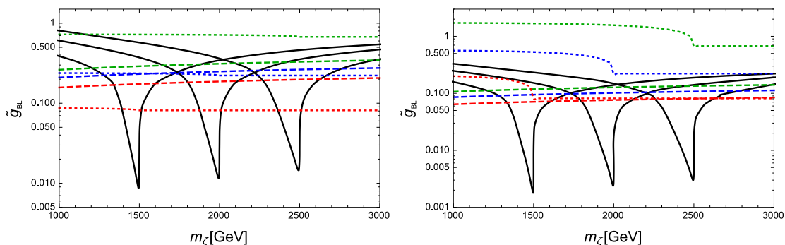
Figure 3. Left panel: plots of \tilde{g}_{BL} vs m_\zeta (solid black lines) that give the observed relic density for M_X = 3, 4 and 5 TeV, respectively, from left to right. Here, we have fixed g_\zeta = \tilde{g}_{BL} . The dotted lines correspond to the ATLAS bounds and dashed lines are the direct detection bounds. The red, blue and green dashed and dotted lines correspond to the bounds for M_X = 3, 4 and 5 TeV for from bottom to top. The dips in the solid lines are where the M_X \simeq 2m_\zeta and we see that constraints from the ATLAS searches for the Z' boson resonance and the direct DM searches are so stringent that only the parameter region near the resonance are allowed for Case (i). Right panel: same as the left panel but for g_\zeta = 6\tilde{g}_{BL} .
