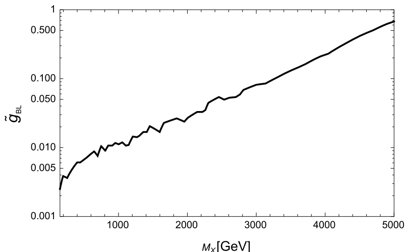
Figure 1. The ATLAS bound on the effective coupling \tilde{g}_{BL} as a function of M_X from figure 5 in ref. [29].
