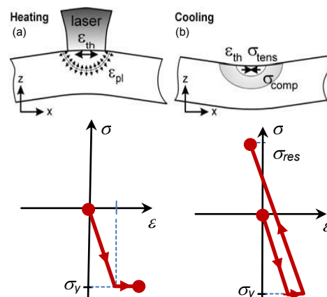
Fig. 1. Residual stress formation model: (a) heating-phase, (b) cooling-phase
