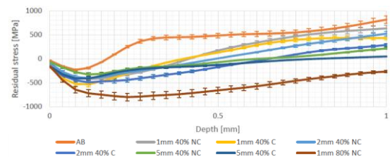
Fig. 4. Tailoring residual stress by laser shock peening [58].
