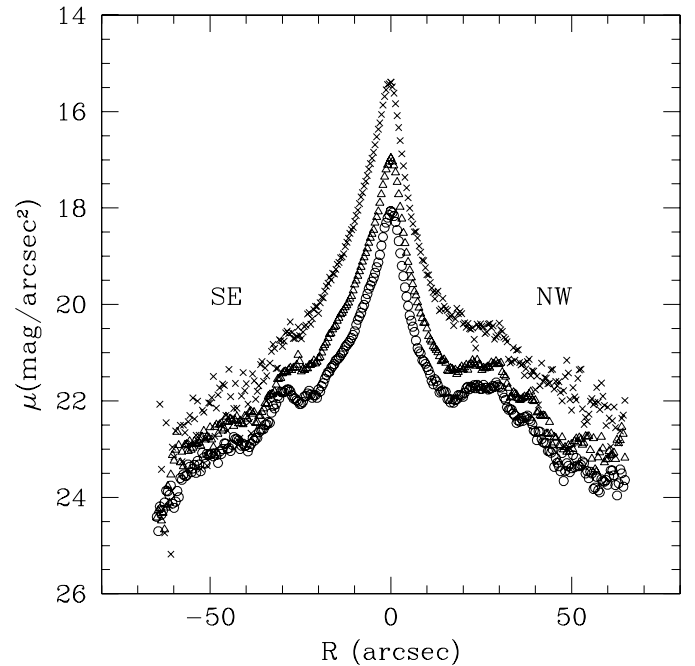
Fig. 5. Surface brightness profiles along the ring major axis, PA = 146°, in B (open circles), V (open triangles) and I bands (crosses).
