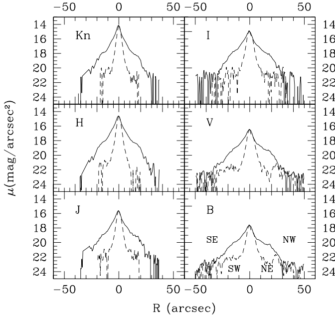
Fig. 4. NIR (left panels) and optical (right profiles) surface brightness profiles along the major, PA = 106°, (continuous line) and minor axis (dashed line) of the central galaxy.
