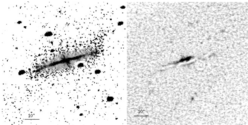
Fig. 3. High frequency residual image for ESO 235-G58 in the H -band ( left panel ) and in the B band ( right panel ). In the B -band image the foreground stars were masked. The darker regions are characterized by a value greater than 1, and lighter regions by a value less than 1. North is at the top and East is to the left.
