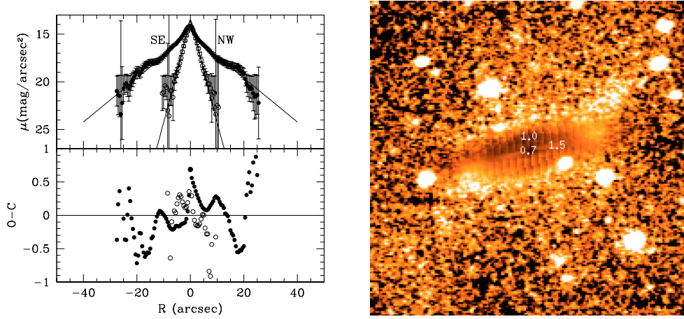
Fig. 14. Left panel: 2D fit of the K -band central galaxy light distribution in ESO 235-G58. The observed light profiles along the major (filled dots), PA = 106^\circ , and minor axis (open dots), PA = 196^\circ , are compared with those derived by the fit (continuous line), which was performed in the K_n band. The orientation, reported on the plot, refers to the major axis. Right panel: residual image obtained as the ratio between the whole image of ESO 235-G58 and the 2D model for the central galaxy in the H band. Units are intensity; whiter colors correspond to those regions where the galaxy is brighter than the model, darker colors correspond to those regions where the galaxy is fainter than the model. Numbers indicate the value of the ratio at that particular isophote. North is up and East is to the left.
