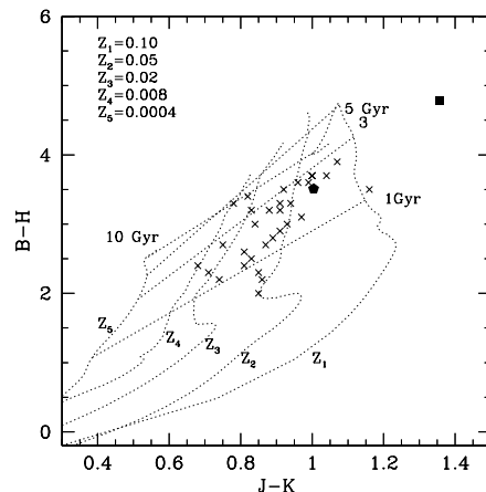
Fig. 13. B-H vs. J-K diagram of the evolutionary tracks for the stellar synthesis models optimized for the central galaxy in ESO 235-G58. The heavier dotted lines correspond to models with a characteristic timescale \tau = 1 \text{ Gyr} . Models are computed for different metallicities as shown on this figure. Light dotted lines indicate loci of constant age for the different models; different ages are reported on the plot. The filled square and pentagon correspond respectively to the nucleus and the outer regions of the central galaxy in ESO 235-G58; crosses are for a sample of spiral galaxies (Bothun et al. 1984).
