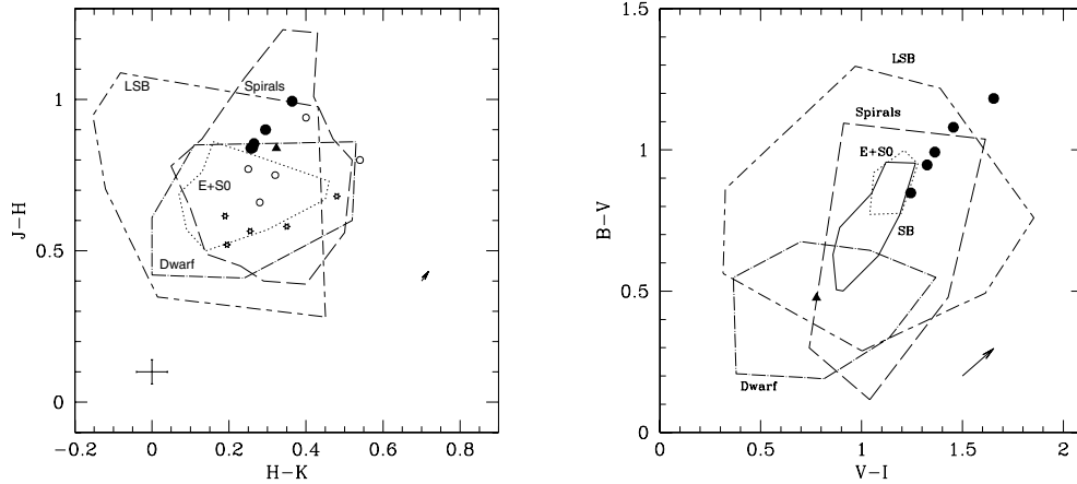
Fig. 12. J-H vs. H-K (left panel) and B-V vs. V-I (right panel) color diagram for the central galaxy (filled circles) and ring (filled triangles) in ESO 235-G58. Open circle indicates the colors of the nuclear regions in PRGs, and open stars indicate the average colors of the host galaxy in PRGs (data are from Iodice et al. 2002b,c). The dotted contour limits the region where the integrated colors of Es and S0s are found; the long-dashed contour limits the integrated colors of spirals; the dashed-dotted contour identifies the integrated colors of the dwarf galaxies and the long dashed–short dashed contour identifies the integrated colors of LSB galaxies and the continuous contour limits the integrated colors of barred galaxies with outer rings. The arrow, in the lower right corner, indicates the reddening vector for galactic dust and the screen model approximation.
