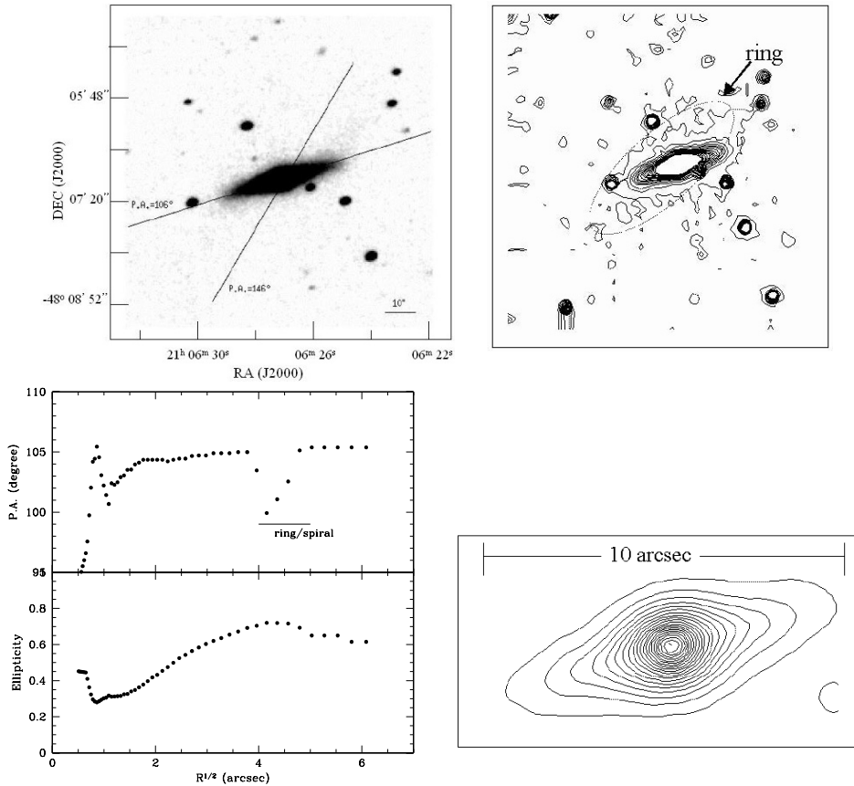
Fig. 2. Top-left panel: H -band image of ESO 235-G58; top-right panel: contour plot, with linear spacing, from the intensity level corresponding to 16.25 \text{ mag/arcsec}^2 to background level. The lines at \text{PA} = 106^\circ and \text{PA} = 146^\circ show apparent major axes of the central galaxy and the outer ring respectively. The image size is 2' \times 2' . North is at the top and East is to the left. In the bottom-left panel are shown the ellipticity and PA profiles along the major axis of the galaxy. In the bottom-right panel is shown the contour plot, with a linear spacing, of the inner regions ( R < 5'' ) of the central galaxy, the last isophote corresponds to 16.45 \text{ mag/arcsec}^2 .
