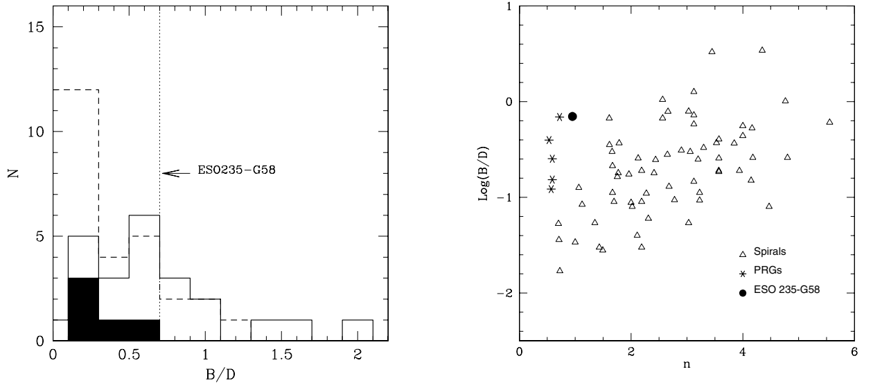
Fig. 15. B/D distribution for the PRGs (filled region), by Iodice et al. (2002b), for early-type galaxies (continuous line), by Bothun & Gregg (1990), and for spiral galaxies (dashed line), by Möllenhoff & Heidt (2001); Khosroshahi et al. (2000). The dotted line indicates the value of B/D derived for ESO 235-G58 (Table 5).
