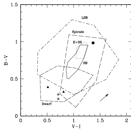
Fig. 10. B - V vs. V - I color diagram for the central galaxy (filled circle) and ring (filled triangles) in ESO 235-G58. Asterisks are the optical colors for the polar structure in NGC 4650A. The dotted contour limits the region where the integrated colors of Es and S0s are found; the long-dashed contour limits the integrated colors of spirals; the dashed-dotted contour identifies the integrated colors of the dwarf galaxies, the long dashed – short dashed contour identifies the integrated colors of LSB galaxies and the continuous contour limits the integrated colors of barred galaxies with outer rings. The arrow, in the lower right corner, indicates the reddening vector for galactic dust and the screen model approximation.
