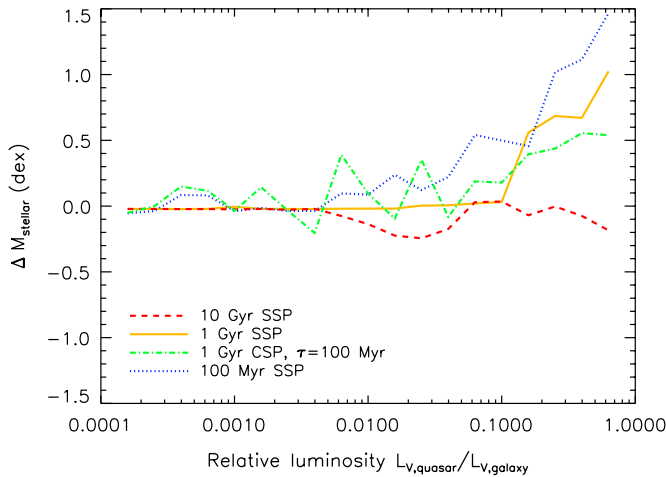
Figure 11. Effect of AGN contribution to stellar mass estimates from optical photometric data. We show the results of a test of the effect of adding a quasar template (from Vanden Berk et al. 2001) to an ensemble of galaxy templates varying the relative V -band luminosity of the quasar and the galaxy template. This test shows that we are able to recover the stellar mass within 0.2 dex for galaxies at least 10 times more luminous in V than the quasar. Stellar mass measurements of host galaxies of brighter quasars degrade as the quasar luminosity approaches the host galaxy.
