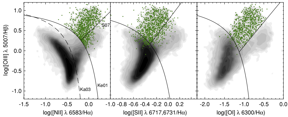
Figure 2. Emission line diagnostic diagrams used for the selection of AGNs from narrow-line fluxes. We use three different diagrams, all of which use the ratio of [O\text{ III}]\lambda 5007/H\beta (vertical axis). From left to right, the horizontal axes are the ratios of [N\text{ II}]/H\alpha , [S\text{ II}]/H\alpha , and [O\text{ I}]/H\alpha . In each panel, we plot those objects that have S/N > 3 in each of the four lines required for the diagram. The gray shading represents the entire galaxy sample, while the green points are the AGN sample selected using these diagrams. In the [N\text{ II}]/H\alpha diagram (left), the dashed line shows the empirical demarcation line between purely star-forming galaxies and the composite region of the diagram determined by Kauffmann et al. (2003a, Ka03). The solid line, labeled Ke01, is the theoretical extreme starburst line of Kewley et al. (2001) beyond which the dominant source of ionization cannot be due to OB stars and must be due to a mechanism other than star formation (AGN, evolved stellar populations or shocks). The solid line labeled S07 is the empirical AGN–LINER distinction defined by Schawinski et al. (2007). The demarcation lines in the [S\text{ II}]/H\alpha and [O\text{ I}]/H\alpha diagrams are taken from Kewley et al. (2006). We select AGN using these diagrams in the following way: if [O\text{ I}]\lambda 6300 is not detected, but [S\text{ II}]\lambda\lambda 6717, 6731 is, then we use the [S\text{ II}]/H\alpha diagram. If neither [O\text{ I}]\lambda 6300 nor [S\text{ II}]\lambda\lambda 6717, 6731 is detected, but [N\text{ II}]\lambda 6584 is, we use the [N\text{ II}]/H\alpha diagram.
