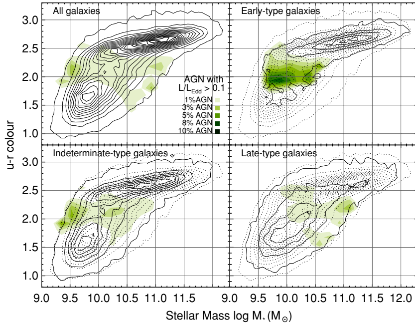
Figure 7. Distribution of the fraction of AGN host galaxies on the color–mass diagram for AGN that have an Eddington parameter L[\text{O III}]/M_{\text{BH}} > 0.7 which corresponds to an Eddington ratio of \gtrsim 0.1 . The layout is identical to Figure 6. This figure shows that the duty cycle of high-Eddington AGN is very low in all galaxy populations except for low mass early types in the green valley. The prominent locus of high duty cycle in massive late types in Figure 6 is therefore not dominated by high-Eddington accretion.
