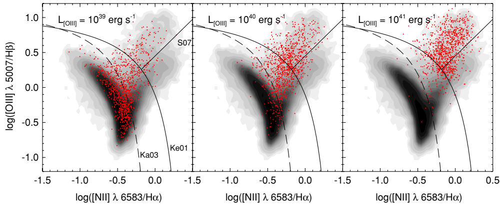
Figure 3. [\text{N II}]/\text{H}\alpha emission-line diagnostic diagrams for all galaxies (shaded) and simulated composite AGN plus star-forming galaxies (red points). The simulated AGN luminosity increases from 10^{39} \text{ erg s}^{-1} in the left panel, to 10^{40} \text{ erg s}^{-1} in the center and 10^{41} \text{ erg s}^{-1} on the right. See Section 3.3 for details. For low values of L[\text{O III}] (left), the nebular emission from star formation can overwhelm the AGN signature, and such low-luminosity AGNs may be missed. At an AGN L[\text{O III}] = 10^{40} \text{ erg s}^{-1} , 12.8% of AGNs move below the empirical starburst line (dashed), while 54.4% move below the extreme starburst line (solid). The result of this test shows that at high luminosities, AGNs are efficiently selected using emission-line diagrams. However, at lower luminosities, star formation may overwhelm the AGN narrow line emission.
