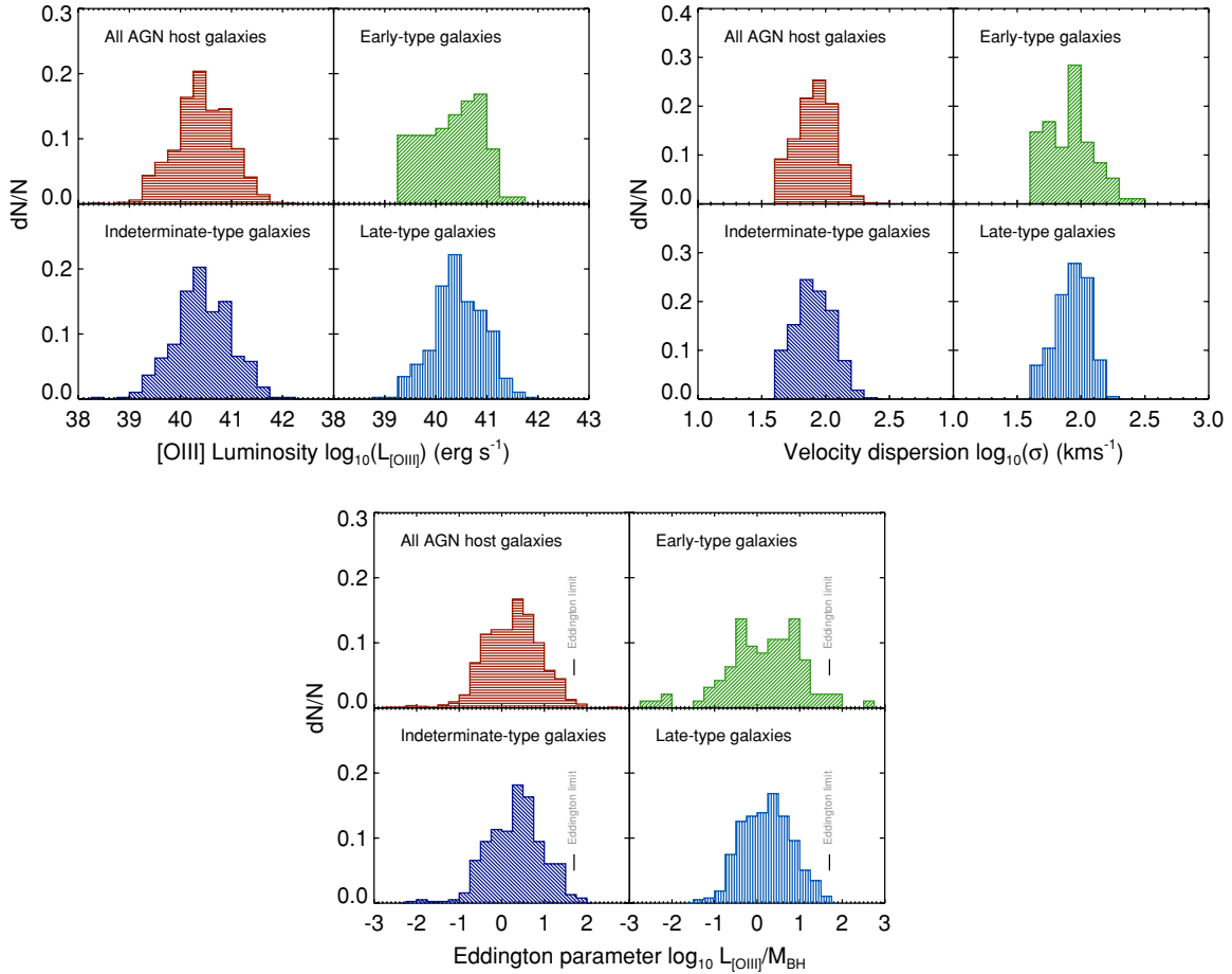
Figure 4. Top left: the distribution of L[\text{O III}] of our AGN sample. Top right: the distribution of stellar velocity dispersions of our AGN sample. Bottom: the distribution of the Eddington parameter L[\text{O III}]/M_{\text{BH}} , combining the values from the plots on the top row via the M_{\text{BH}}-\sigma relation. We indicate the approximate value of the Eddington limit in each panel. In each of the panels, we show the distribution of the entire AGN population in the top-left, while the remaining panels show the L[\text{O III}] distribution split by host morphology.
