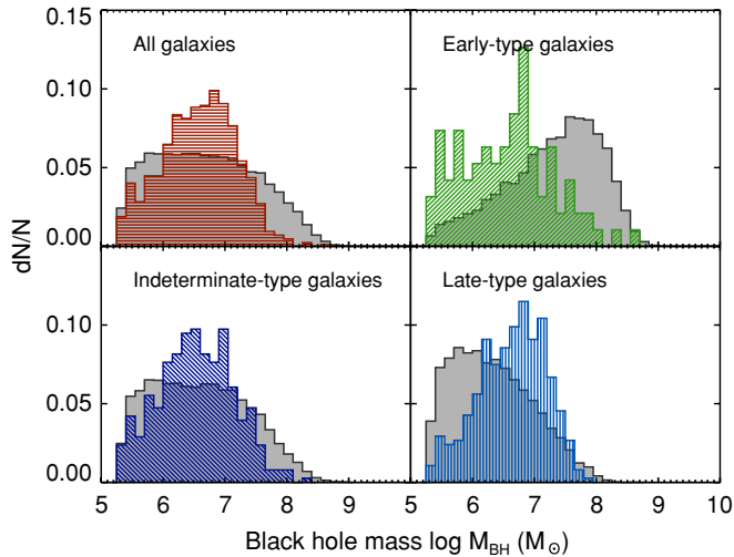
Figure 8. Distribution of supermassive black hole masses M_{\text{BH}} for both normal galaxies and AGN host galaxies as a function of morphology. In each panel, we show histogram of M_{\text{BH}} for the normal galaxy population (gray, solid) and the AGN only (colored, dashed). Both here and in Figure 9, we plot only objects where the measured velocity dispersion is greater than 40 \text{ km s}^{-1} (corresponding to \log(M_{\text{BH}}) \sim 5.3 ; Tremaine et al. 2002). The mean and median black hole masses of both early- and late-type AGN host galaxies are very similar (see Table 2), but when their distributions are compared to those of normal galaxies, large differences become apparent. Among the early-type galaxy population, it is preferentially those galaxies with lower black hole masses that are AGNs, while the opposite is the case for the late-type galaxies.
