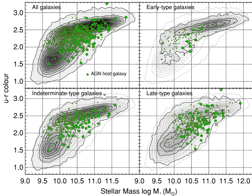
Figure 5. Distribution of AGN host galaxies on the u - r color–mass diagram (green dots). Top left: galaxies of all morphologies; top right: early-type galaxies; bottom left: indeterminate-type galaxies; bottom right: late-type galaxies. The solid, shaded contours in each case show the galaxy population, on top of which we plot the individual AGN as green points. The large points are those AGN with L[\text{O III}] > 10^{41} \text{ erg s}^{-1} . In the panels for each specific morphology class, we only plot AGN host galaxies in that specific class. Furthermore, to guide the eye, we overplot the contours of all galaxies from the top left panel as gray dotted contours. The contour levels in all panels are linear and represent the same contour levels. From this figure, we see that AGN host galaxies preferentially have green host galaxy colors and a range of stellar masses—but that this range is clearly morphology dependent. That is, AGN host galaxies are a very particular subset of normal galaxies, and the way in which they are separated depends on morphology.
