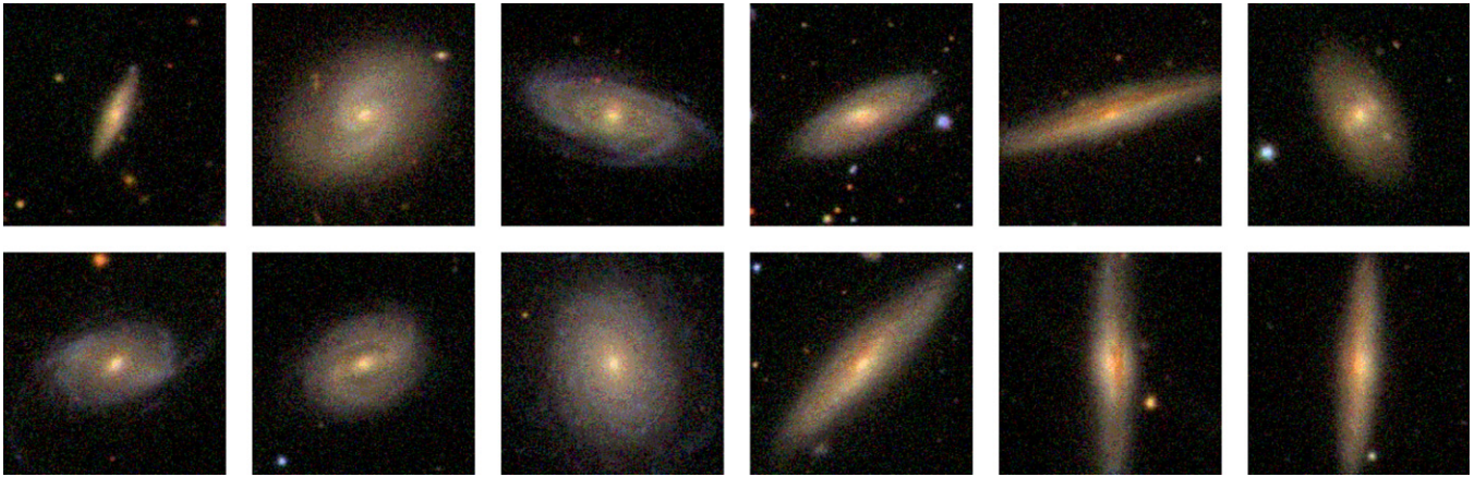
Figure 10. Example SDSS gri images 80'' \times 80'' in size of late-type AGN host galaxies with stellar masses above 10^{11} M_{\odot} . These images illustrate that massive late-type AGN hosts are not massive bulges with a small disk (S0 or Sa), but rather have small bulges and massive disks. (A color version of this figure is available in the online journal.)
