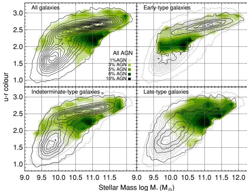
Figure 12. Same as Figure 6, but for all objects classified as Seyfert or LINER with L[\text{O III}] > 10^{40} \text{ erg s}^{-1} . This figure illustrates that the inclusion of the small fraction of LINERs that have high [\text{O III}] \lambda 5007 luminosities does not substantially change the results presented in this work.
