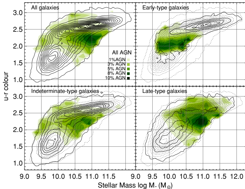
Figure 6. Distribution of the fraction of galaxies that host AGN on the color–mass diagram. The layout of this figure is similar to that in Figure 5, though for clarity, we do not shade the contours of the galaxy population. The filled contours represent the AGN fraction, which has been calculated in cells of size 0.175 dex in stellar mass and 0.125 mag in u - r color. We consider only cells that contain at least 50 objects to minimize noise. The legend in the top left panel relates the shading level to the AGN fraction. As we argue in Section 4, the AGN fraction is a proxy for the AGN duty cycle. This figure reveals in stark terms that those galaxy populations that only very specific sub-populations of galaxies have a high AGN duty cycle: in the early-type population, it is only low-mass galaxies in the green valley that have a high AGN duty cycle. Early-type galaxies on the red sequence, regardless of mass, do not have an appreciable duty cycle. In the late-type population, it is massive galaxies that have an AGN high duty cycle. The duty cycle peaks strongly in a “sweet spot” in the green valley. The high mass of late-type AGN host galaxies is somewhat misleading, as they have similar black hole masses, and therefore bulge masses, to the early-type AGN hosts. Their higher stellar mass is therefore due to a disk, rather than a bulge (see Table 2). Example images are shown in Figure 10. The Milky Way galaxy most likely resides in the “sweet spot” for the AGN duty cycle in late types.
