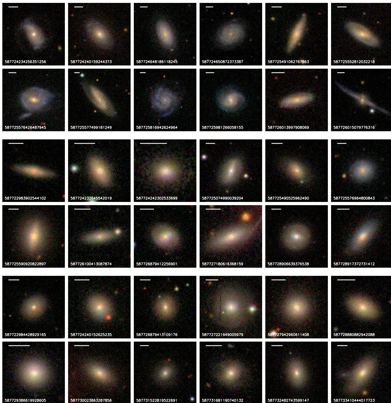
Figure 1. Example images of AGN host galaxies in three morphology classes. The top two rows are late-type host galaxies, the middle rows are indeterminate-type and the bottom two rows are early-type host galaxies. In the top left of each image, we show a bar of 5 kpc length at the redshift of the object. In the bottom, we provide the SDSS object ID.
