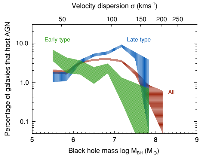
Figure 9. Fraction of supermassive black holes that are growing in the local universe. We plot the black hole mass M_{\text{BH}} vs. the fraction of galaxies that host an AGN. The errors on the fraction are Poisson errors. We plot the AGN fraction for the entire sample as well as for galaxies of specific morphology classes: (red) all; (green) early types; (blue) late types. This plot elaborates on the trend seen in Figure 8 and shows the relative incidence of AGN in galaxies of early- and late-type morphology. The AGN fraction—and therefore the duty cycle—in early-type galaxies is heavily skewed toward low black hole masses. In late-type galaxies, the AGN fraction is skewed toward higher black hole masses, potentially with a drop at the highest masses.
