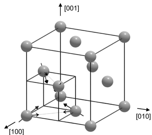
FIG. 4. Three-dimensional spin structure of FeMn according to the \langle 111 \rangle model. The projection of the spin directions onto the (001) surface are also indicated by black arrows.
