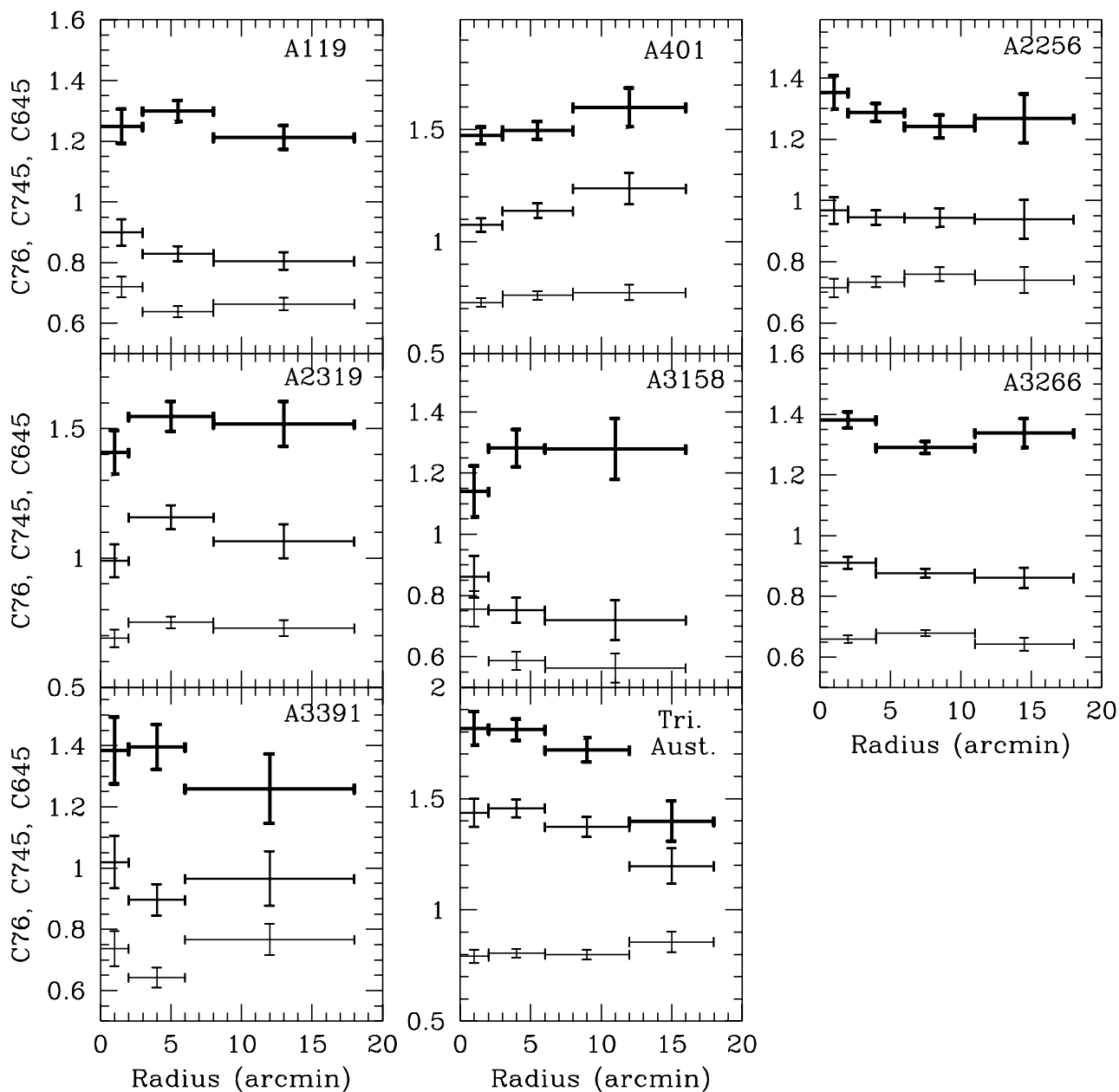
FIG. 4.—Radial color profiles for clusters with kT > 5 keV and \dot{M} < 50 M_{\odot} \text{ yr}^{-1} . The notation is the same as that for Fig. 3.
