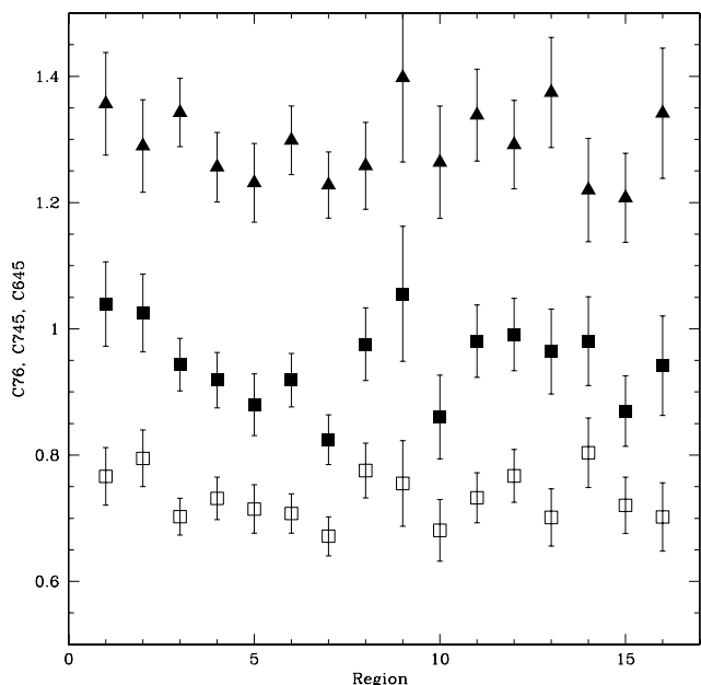
FIG. 7.—Azimuthal color profiles for A2256. Regions 1–8 represent 45^\circ sectors running counterclockwise from north for the inner 5' . Regions 9–16 represent the same sectors for the 5' – 9' radial bin.
