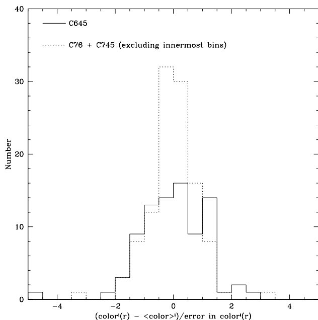
FIG. 9.—Distribution of [color^i(r) - \langle color \rangle^i] / [\text{error in } color^i(r)] values for C645 (solid lines) and C76 + C745 (dotted lines) for each spatial bin of each individual cluster i in the sample. For C76 + C745, the innermost spatial bins were excluded, since they contain cooling gas in many of the clusters. For both distributions, the shape is approximately Gaussian with a mean near zero and a dispersion close to unity. For C645 this implies that our contamination source removal and background subtraction are accurate. For C76 + C745, this result implies that the consistency between the outer two spatial bins is not the result of merging together rapidly increasing and rapidly decreasing individual color profiles.
