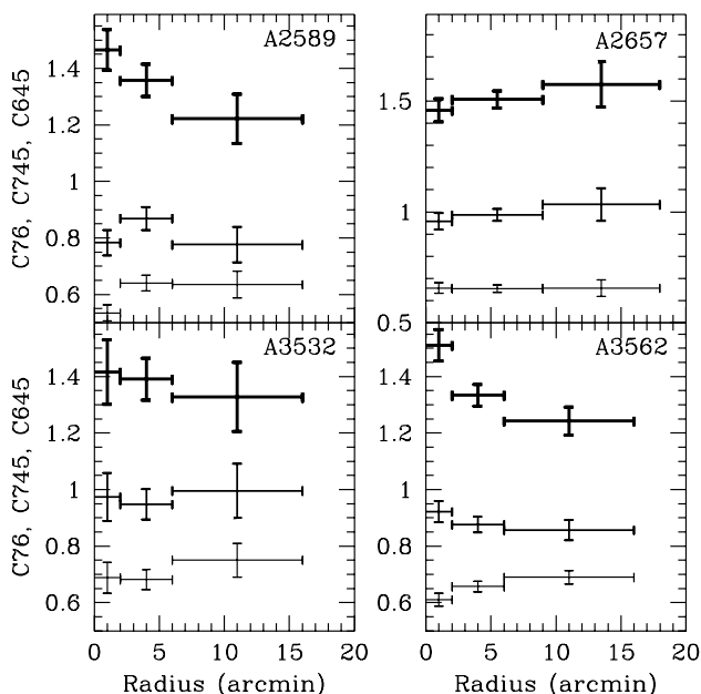
FIG. 6.—Radial color profiles for clusters with kT < 5 keV and \dot{M} < 50 M_{\odot} \text{ yr}^{-1} . The notation is the same as that for Fig. 3.
