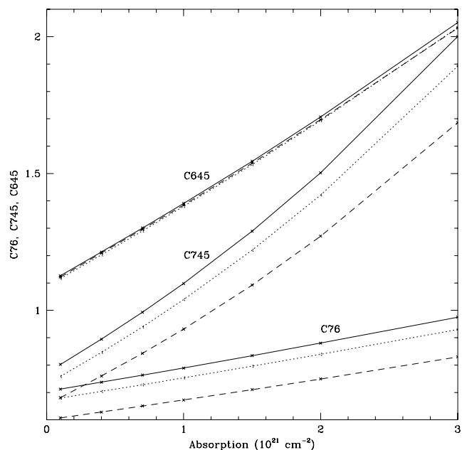
FIG. 2.—Model color profiles as a function of absorbing column density. The top lines are C645, the middle lines are C745, and the bottom lines are C76. The metallicity of the models is 40%. For each color, the solid line represents the 10 keV track, the dotted line represents the 6 keV track, and the dashed line represents the 3 keV track. The relative ratios of colors at different temperatures are independent of column density.
