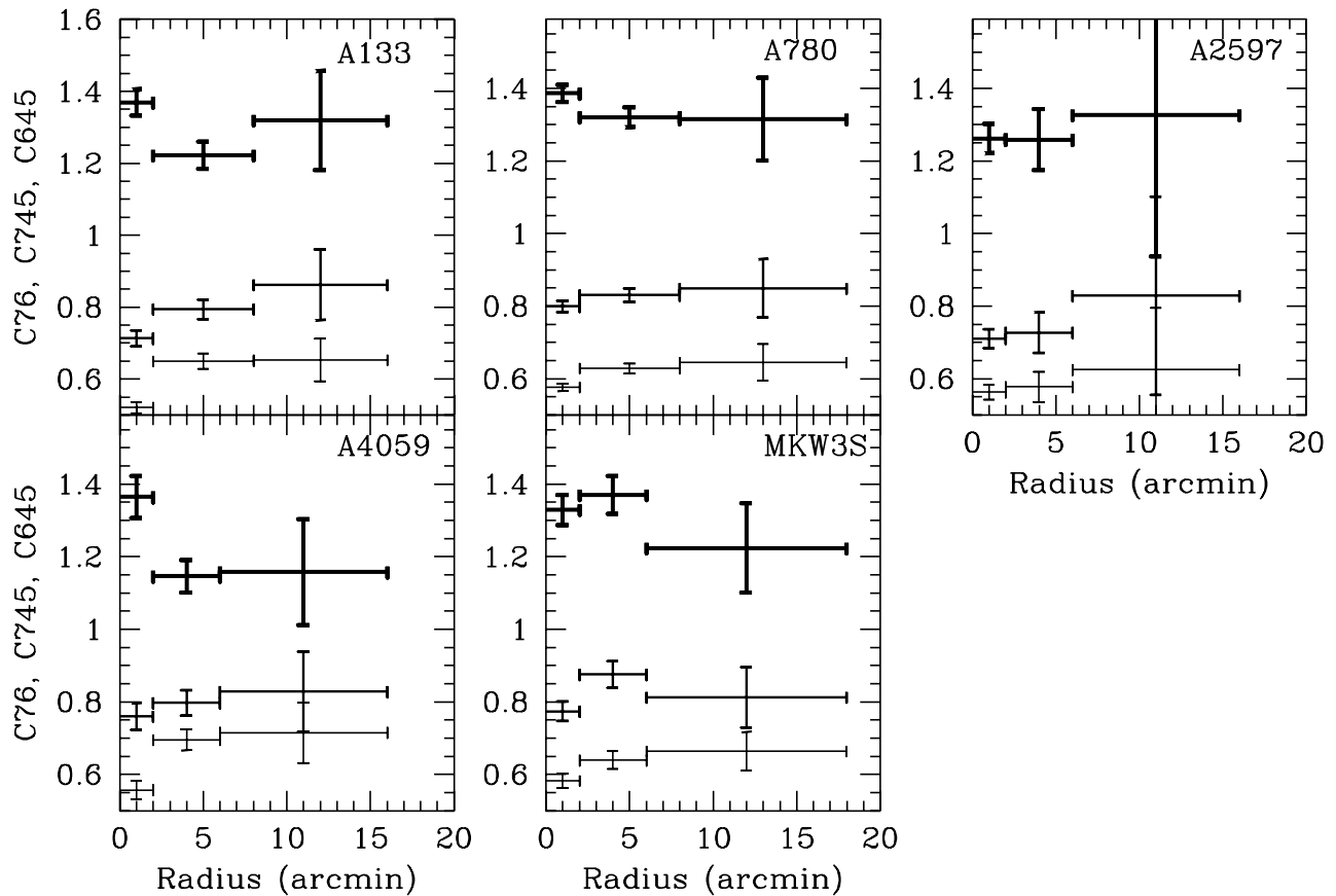
FIG. 5.—Radial color profiles for clusters with kT < 5 keV and \dot{M} > 50 M_{\odot} \text{ yr}^{-1} . The notation is the same as that for Fig. 3.
