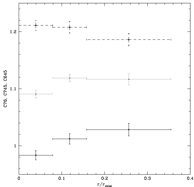
FIG. 8.—Composite radial color profiles for all 26 clusters in the sample. The C76 profile is shown in solid lines, C745 is shown in dotted lines, and C645 is shown in dashed lines. The errors represent the uncertainty in the mean for the sample.
