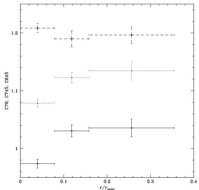
FIG. 10.—Composite radial color profiles for all cooling flow clusters with cooling rates higher than 50 M_{\odot} \text{ yr}^{-1} . The notation is the same as that in Fig. 8.
