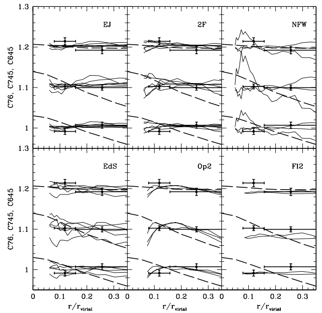
FIG. 14.—Comparison of the colors of the temperature profiles from six cosmological models taken from Evrard et al. (1996; solid lines ) with those of the outer two bins of the composite profile for all clusters in our sample and with the best-fit polytropic relation between temperature and radius from M98 ( \gamma = 1.24 , long-dashed line ). For clarity, the C745 and C645 profiles have been multiplied by 1.1 and 1.2, respectively. For each cosmology, the models cover a range of temperatures and masses. The polytropic relation of M98 is inconsistent with both the models and the ROSAT data.
