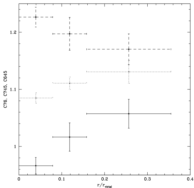
FIG. 12.—Composite radial color profiles for all clusters with kT < 5 keV. The notation is the same as that in Fig. 8. A definite decline in C645 is evident, which is indicative of a negative radial abundance gradient.
