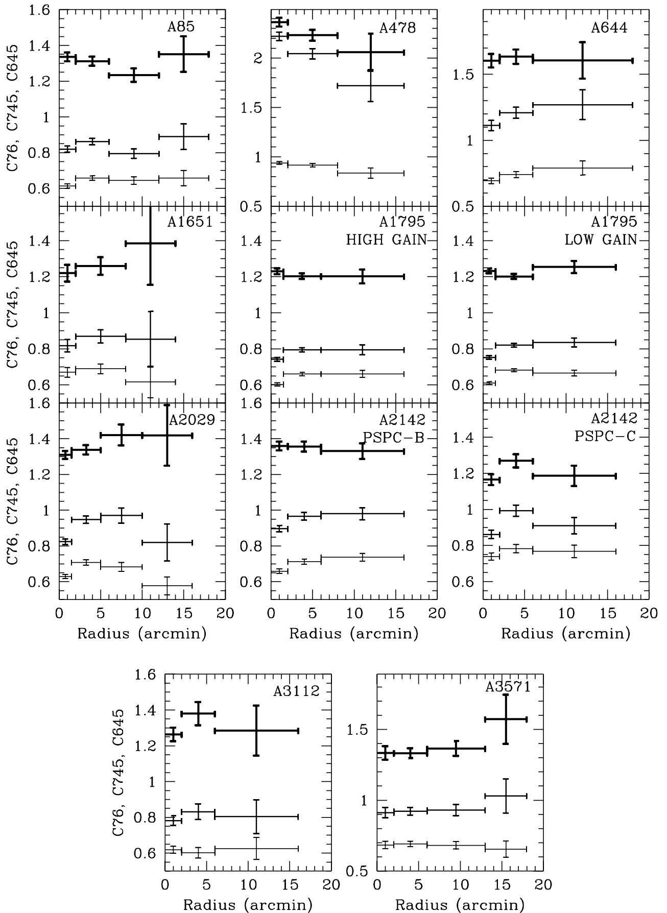
FIG. 3.—Radial color profiles for clusters with kT > 5 keV and \dot{M} > 50 M_{\odot} \text{ yr}^{-1} . The top profile in each panel is C645, the middle is C745, and the bottom is C76.
