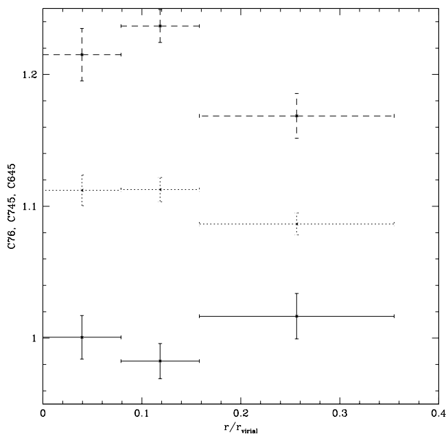
FIG. 11.—Composite radial color profiles for all non-cooling flow clusters. The notation is the same as that in Fig. 8.
