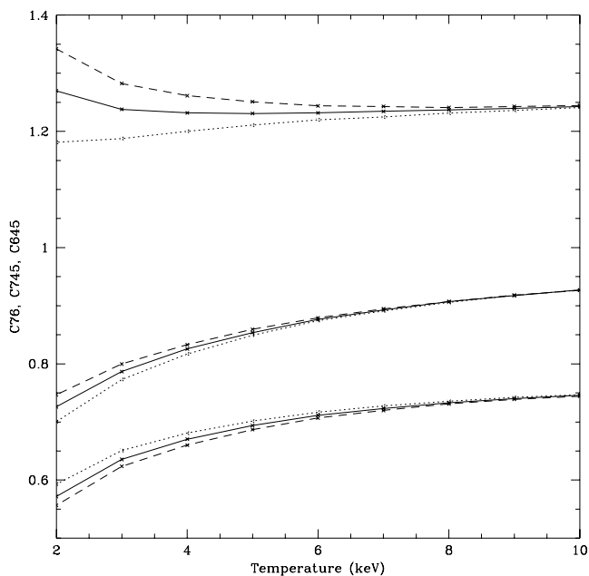
FIG. 1.—Model color profiles derived from the PSPC-B (low gain) response for a variety of Raymond-Smith spectral models. The top lines are C645, the middle lines are C745, and the bottom lines are C76. For each color, dashed lines represent models with 60% metallicity, solid lines represent 40% metallicity, and dotted lines represent 20% metallicity. Metallicity has a small effect on C645 at low temperatures, but it has a minimal effect on C76 and C745. Note that the effect of metallicity on C745 and C76 is reversed. These models illustrate that C76 and C745 are sensitive to changes in temperature, whereas C645 is insensitive to changes in temperatures above 5 keV or near 40% metallicity.
