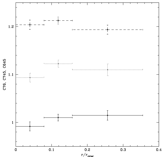
FIG. 13.—Composite radial color profiles for all clusters with kT > 5 keV. The notation is the same as that in Fig. 8. The decline in C645 seen in the low-temperature clusters is not seen here, since C645 is not sensitive to abundance changes at higher temperatures.
