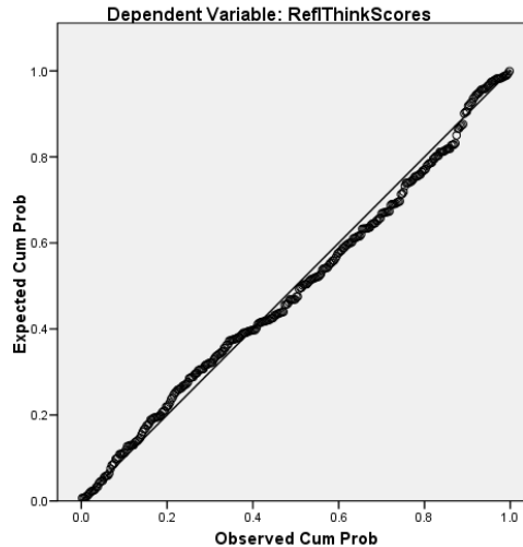
Figure 1: Regression Line
