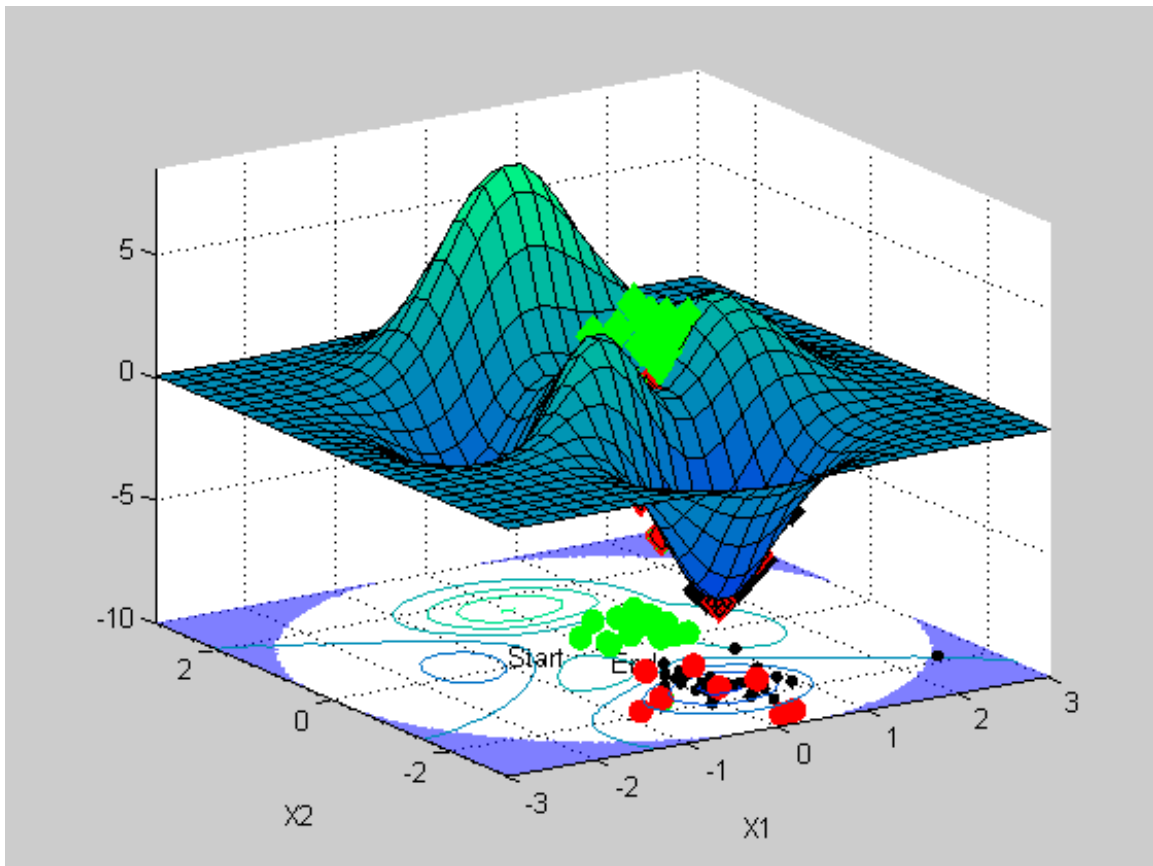
Figure 3: Stochastics
